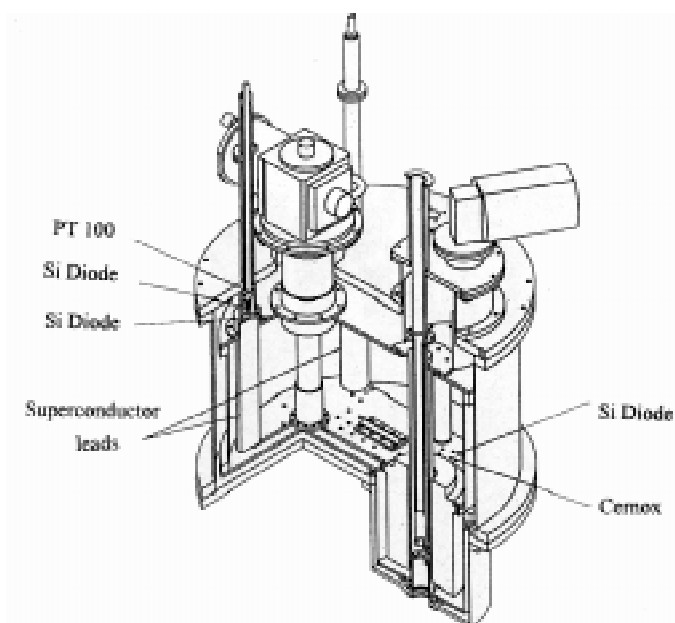
Figure 2. Three-dimensional view of the magnet showing its interior parts.
